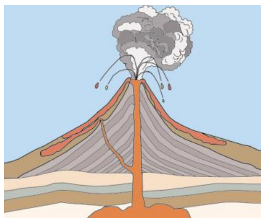
volcan
