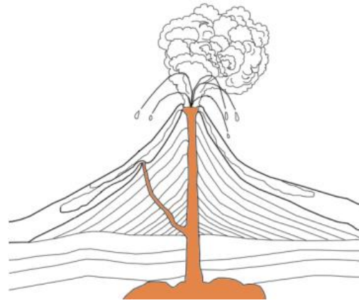
magma
