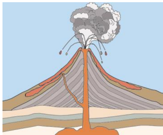
volcan
